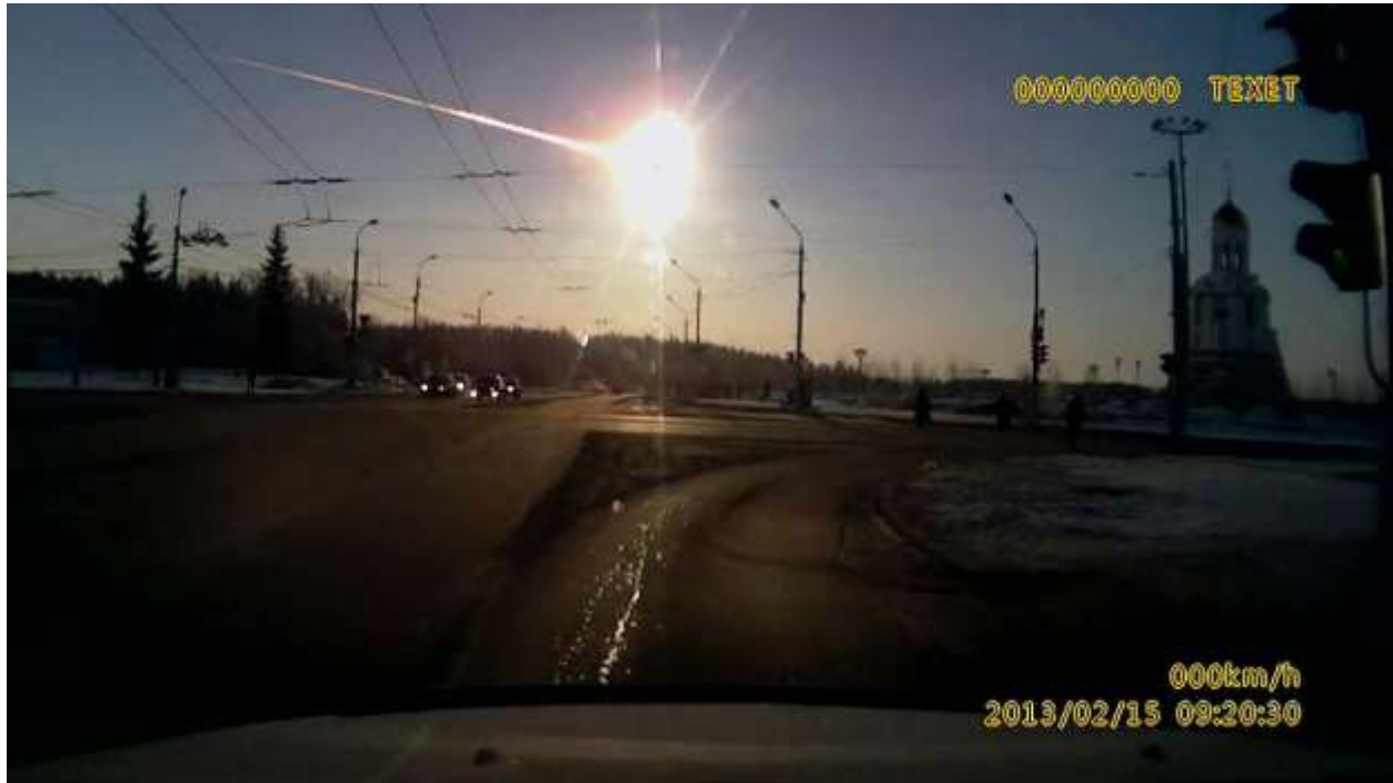
Figure 2 A meteor that created an airburst over Chelyabinsk, Russia in 2013. 4
