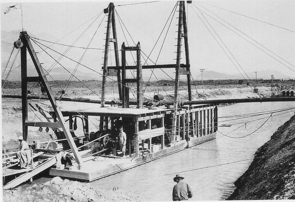
Dredge No. 1, working in Owens Valley.
