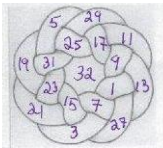
Figure 1. Biquadratic temporal eternity module of all numbers coming from the future!
