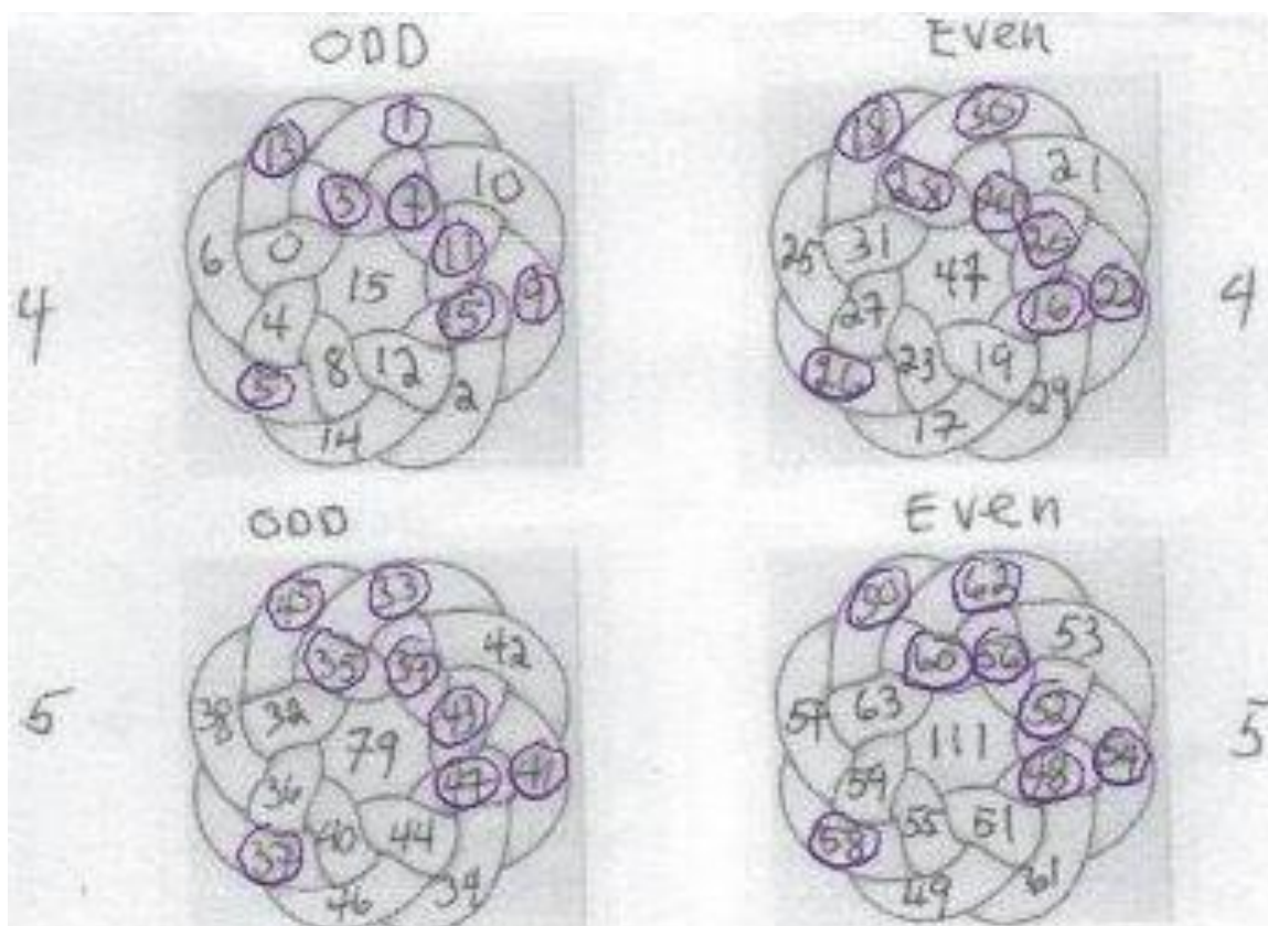
Figure 1. Biquadratic temporal eternity module of all numbers coming from the future!
