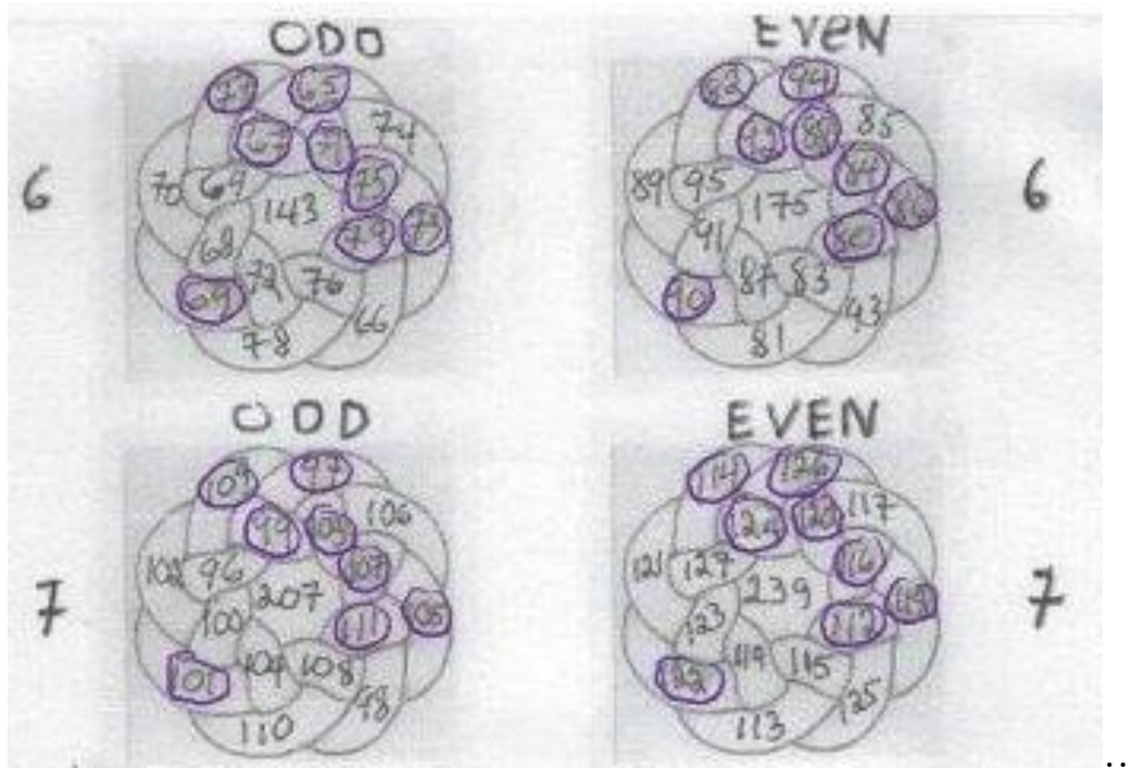
Figure 2. Eight sets of reciprocal time-reversal temporal eternity modules.
