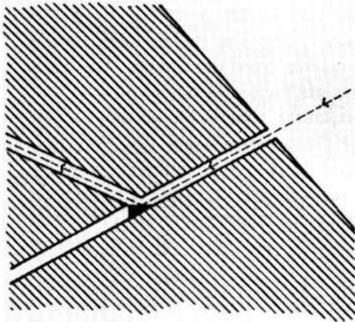
Figure 4 REFLECTING POOL AT THE JUNCTION OF THE DESCENDING AND ASCENDING PASSAGES. By plugging the junction and placing water in it, light could be reflected upward. By looking down the Descending Passage into the reflecting pool, an ancient observer could have noted the exact moment of a star's transit. The same system is used today at the U.S. Naval Observatory where the daily transit of stars is noted by their reflection in a pool of mercury. Source: Peter Tompkins, Secrets of the Great Pyramid (New York: Harper Colophon Books. 1971)
